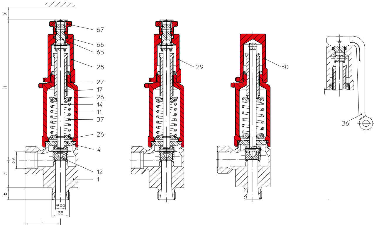
Fig. ... 961 closed lifting device
