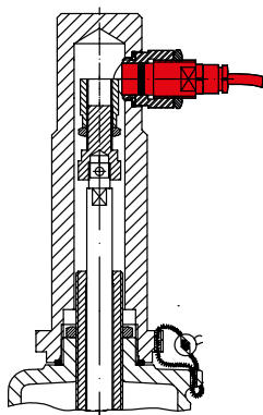
Proximity switch
