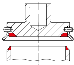
Lock bushing
