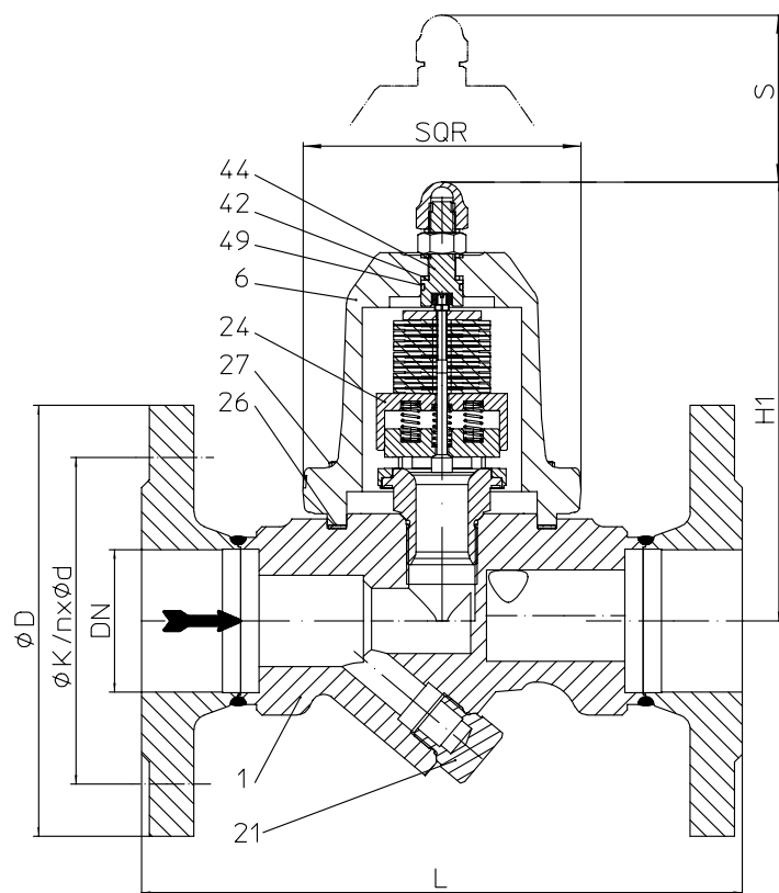
Fig. 650....1 with flanges
