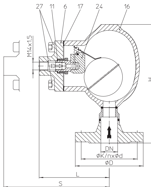
Fig. 656...1 with flange
