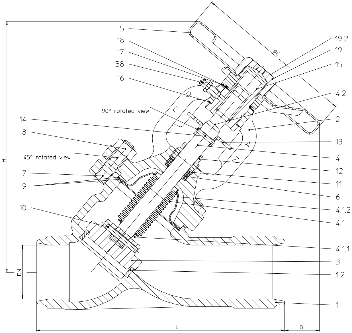
Plug-Spindle connection ≥ DN150
