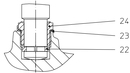
Plug-Spindle connection ≥ DN150
